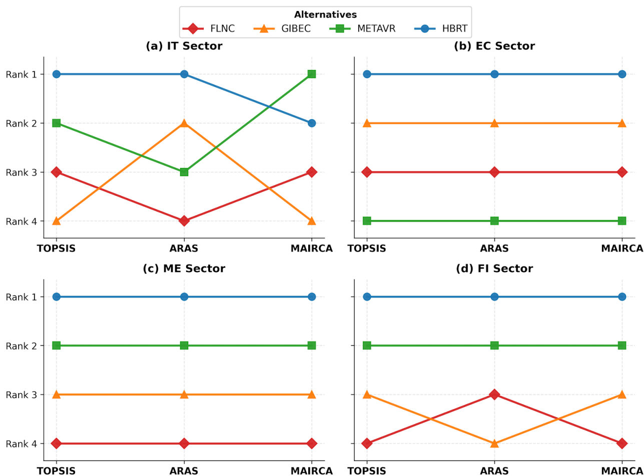
Fig. 11. Comparative Results
